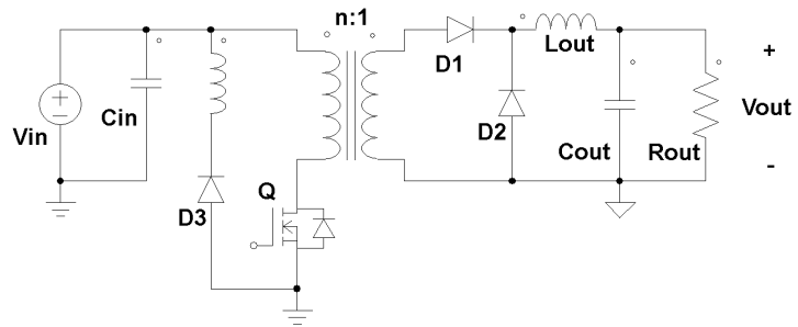
Figure 1.2. Forward Converter Circuit.
