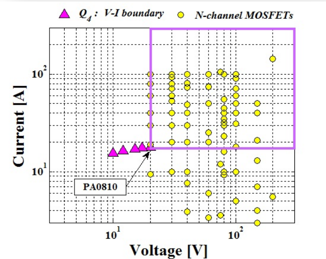
Figure 5.5 AR for MOSFET Q_4 according to PA0810 transformer.
