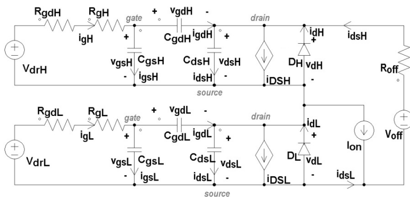
Figure 4.2 Circuit model: case study.
