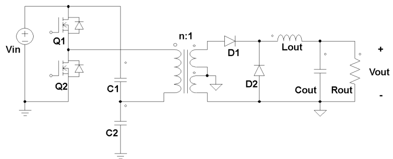
Figure 1.5 Half-Bridge Converter Circuit.
