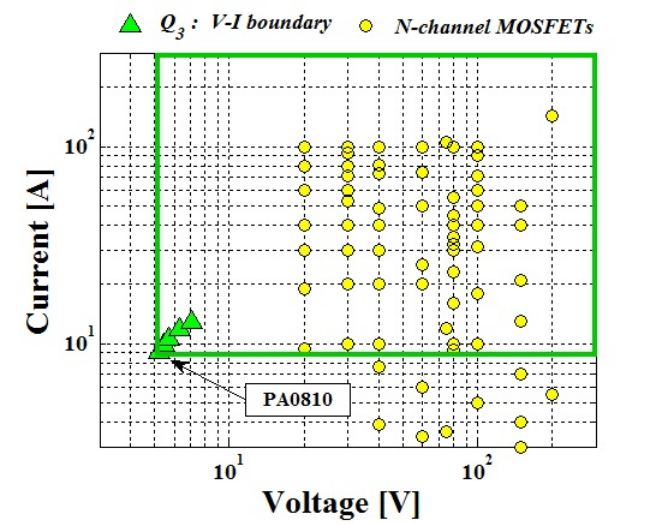
Figure 5.4 AR for MOSFET Q_3 according to PA0810 transformer.
