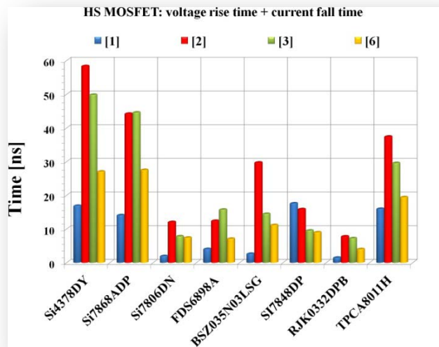
Figure A4. HS MOSFET switching time: turn-off.
