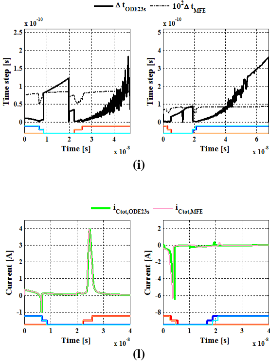
Figure 4.7 (Cont.) MFE and ODE23s with AbsTol=1e-7 results for case #2: (i) ODE23s and MFE time steps during simulations; (I) total capacitive currents flowing through HSM channel during commutations.
