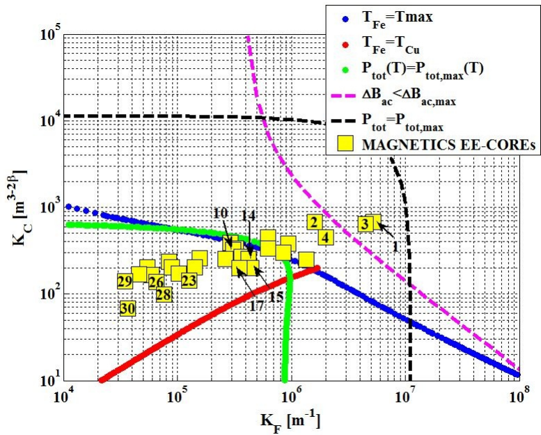
Figure 3.10 ABCs for n_M=2 in (K_f, K_c) plane.
