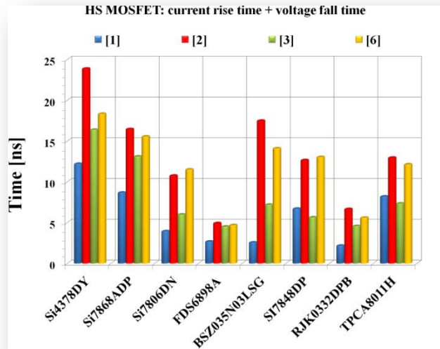
Figure A3. HS MOSFET switching time: turn-on.
