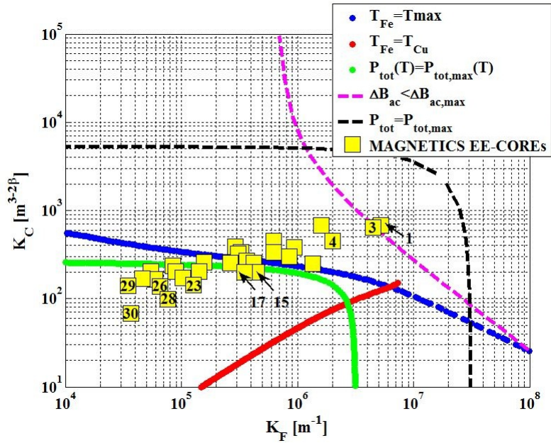
Figure 3.9 ABCs for n_M=3 in (K_f, K_c) plane.
