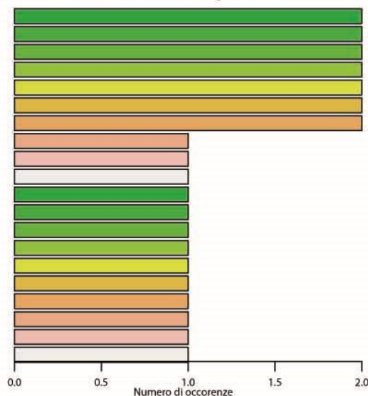
Inchieste Sociali 1913 – Trigrams (tau)
