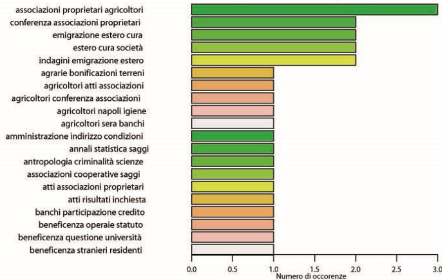
Inchieste Sociali 1890 – Trigrams (tau)
