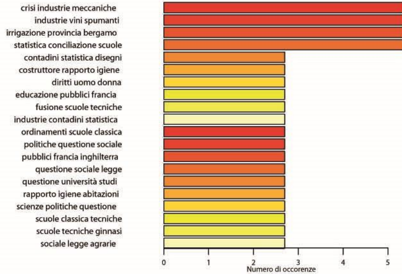
Inchieste Sociali 1891 – Trigrams (tau)
