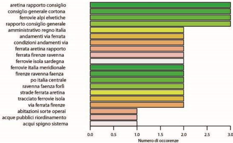
Inchieste Sociali 1861 – Trigrams (tau)
